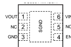
DFN2x2-6L
