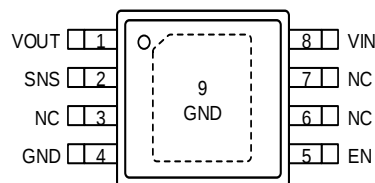
DFN2x2-8L &amp; DFN3x3-8L
