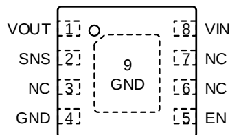
DFN2x2-8L &amp; DFN3x3-8L
