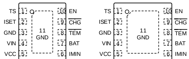
DFN2x2-10L &amp; DFN2x3-10L
